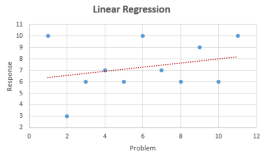
Figure 4: Linear regression.
